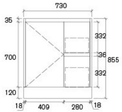
SK32-750W-SD Size: 730x355x855mm
